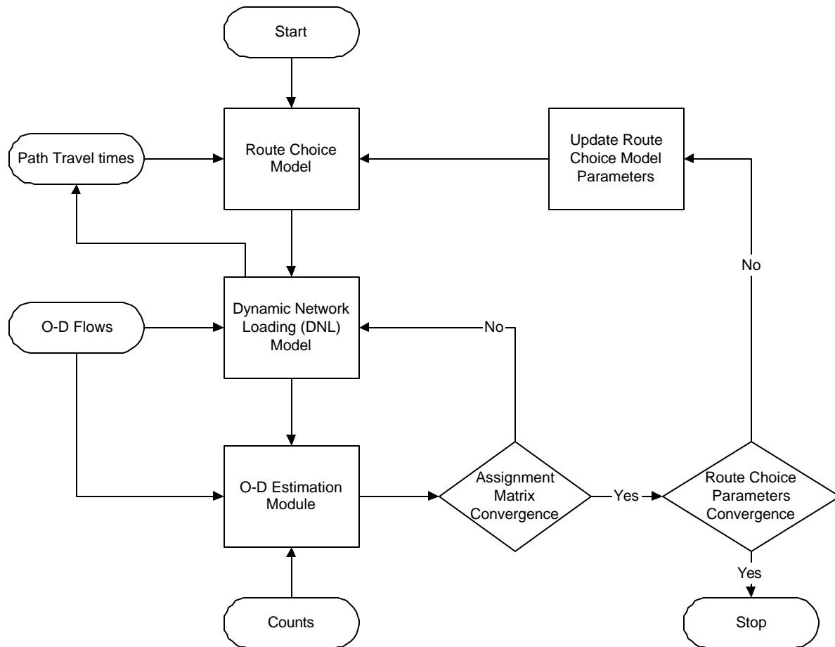
Figure 2-3: Iterative Demand Calibration Framework.
