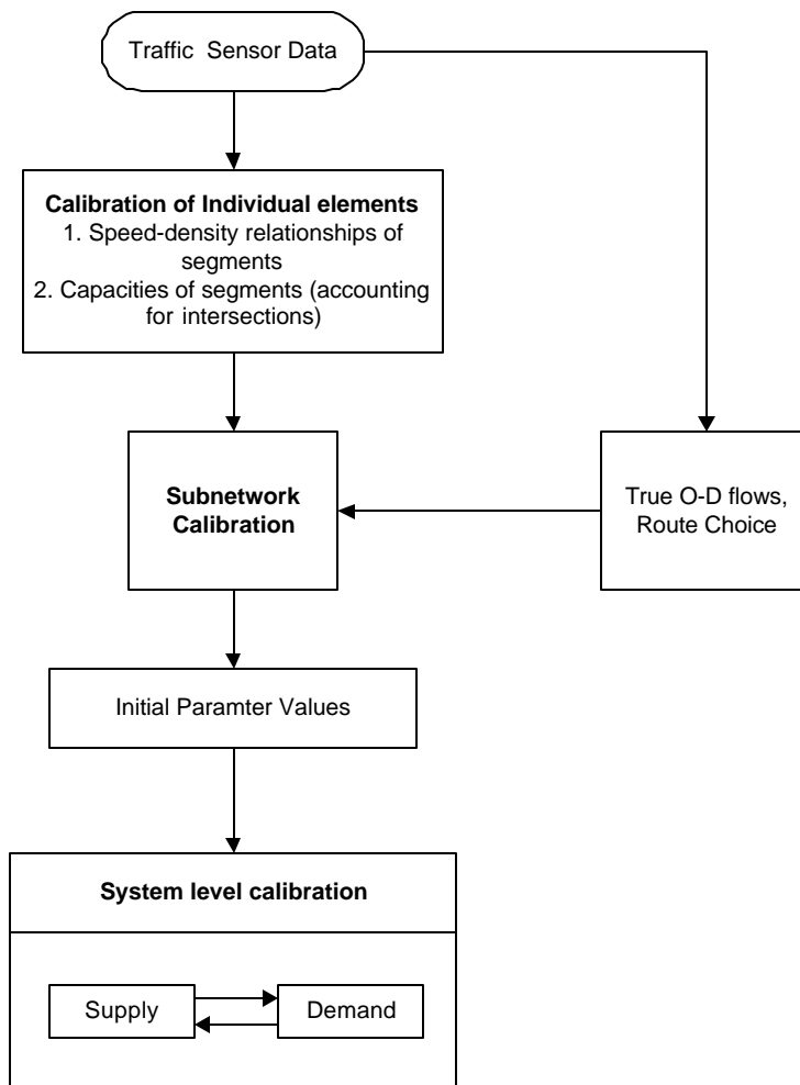
Figure 2-4: Three-stage Supply Calibration
