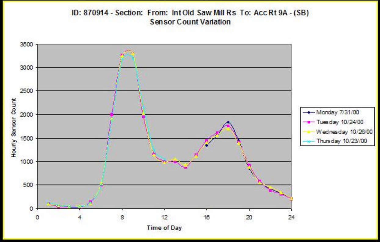
Figure 4-6: Sensor Count Variation for a Parkway (Saw Mill River Parkway, North and South Bound) Sensor
