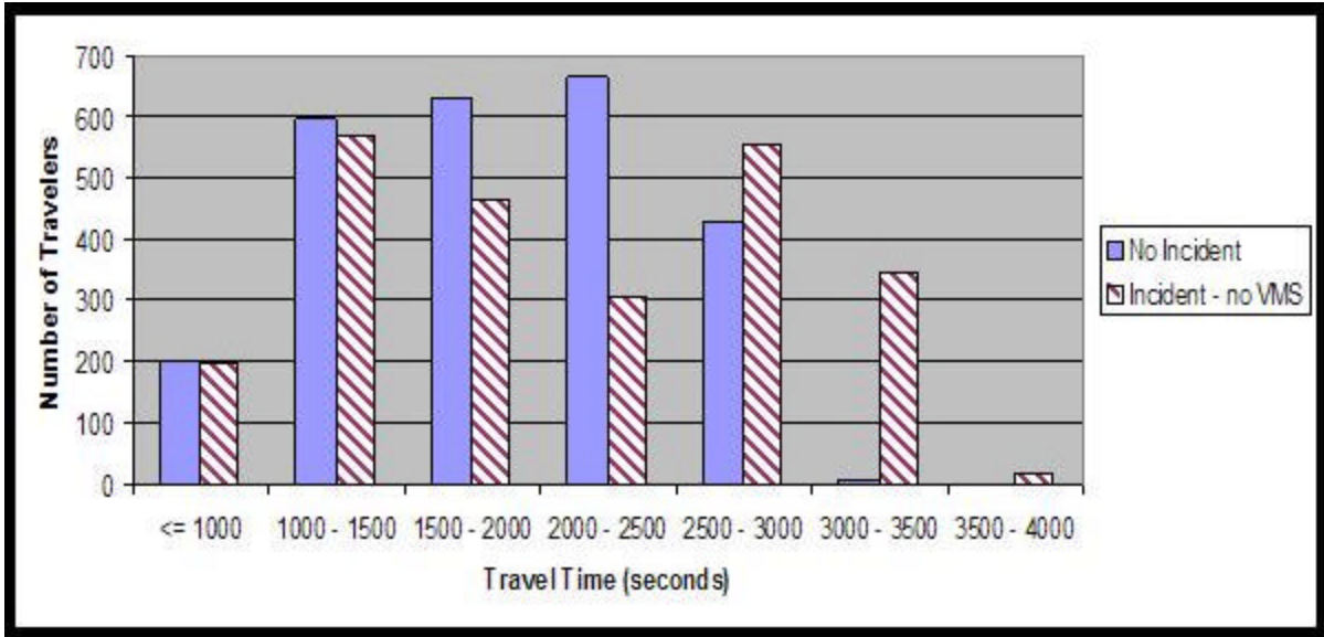
Figure 5-17: Impact of Incident. Frequency of Experienced Travel Times for all OD pairs “1, 2, 3, 4, 8 – 9, 10, 11”.
