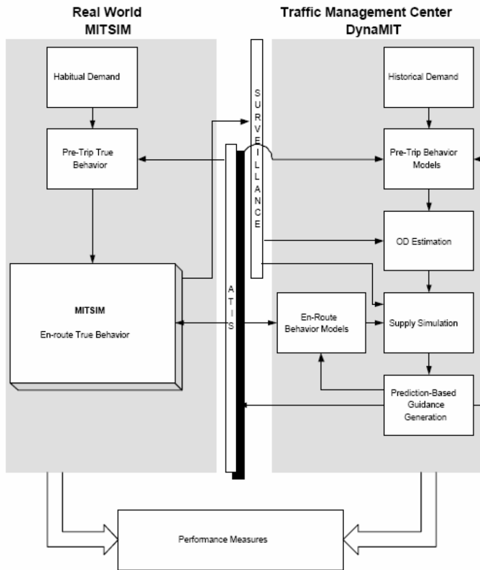
Figure 2-3 Dynamic Traffic Management Evaluation Framework using DynaMIT
