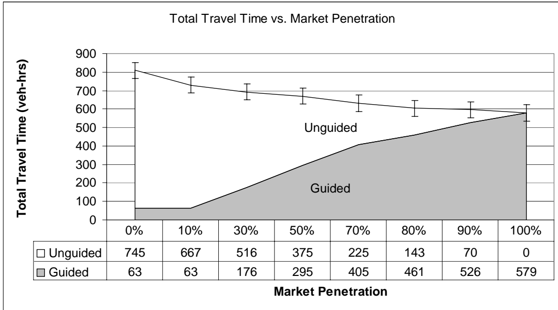
Figure 4-5 Total Travel Time vs. Market Penetration
