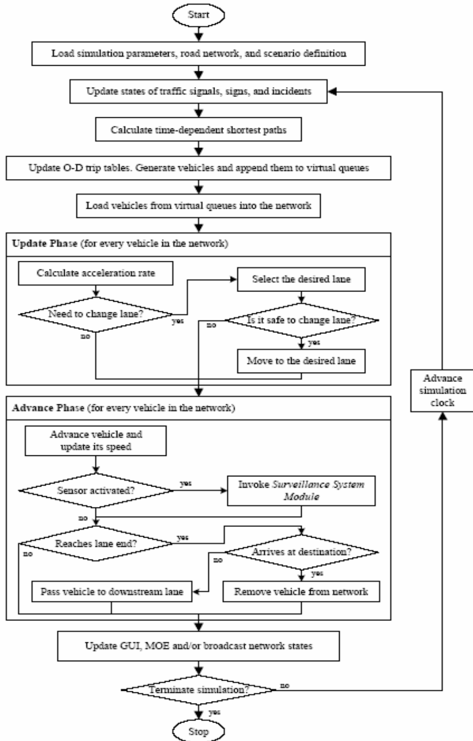
Figure 3-2 MITSIM Clock-Based Operation
