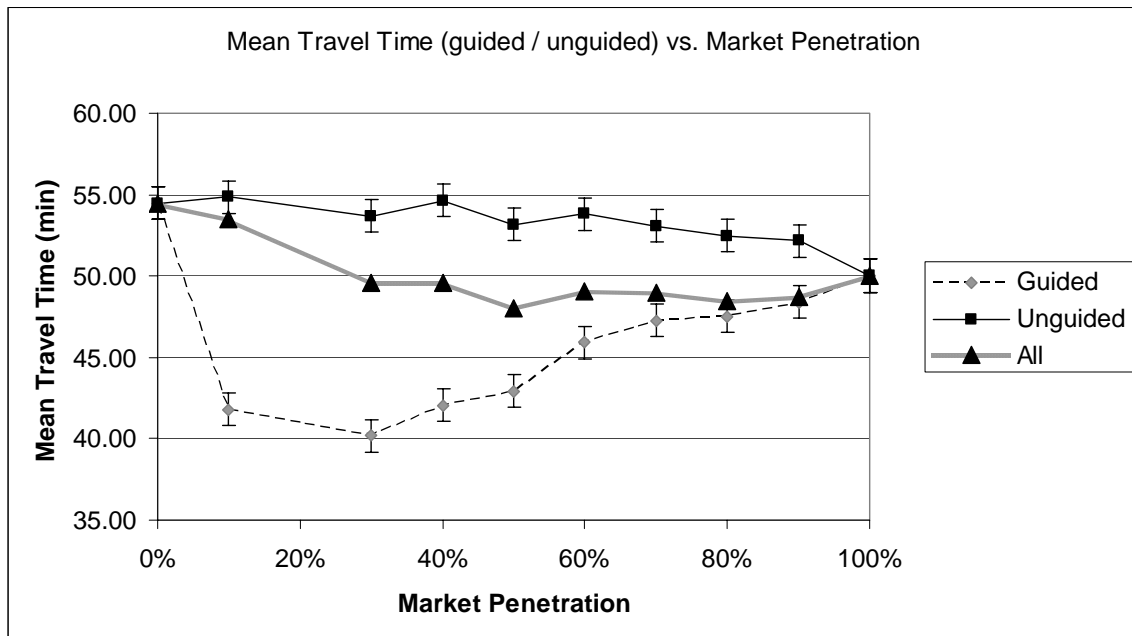
Figure 4-7 Distributional (guided/unguided) Mean Travel Time vs. Market Penetration (High Demand)
