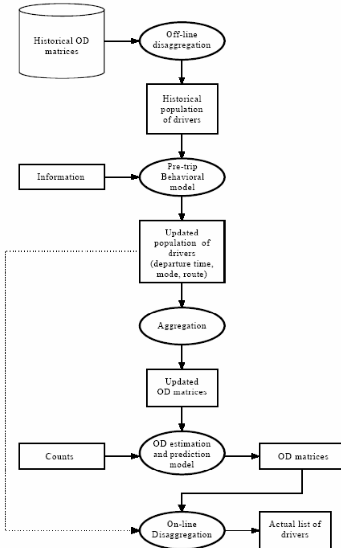
Figure 3-5 DynaMIT Demand Simulation
