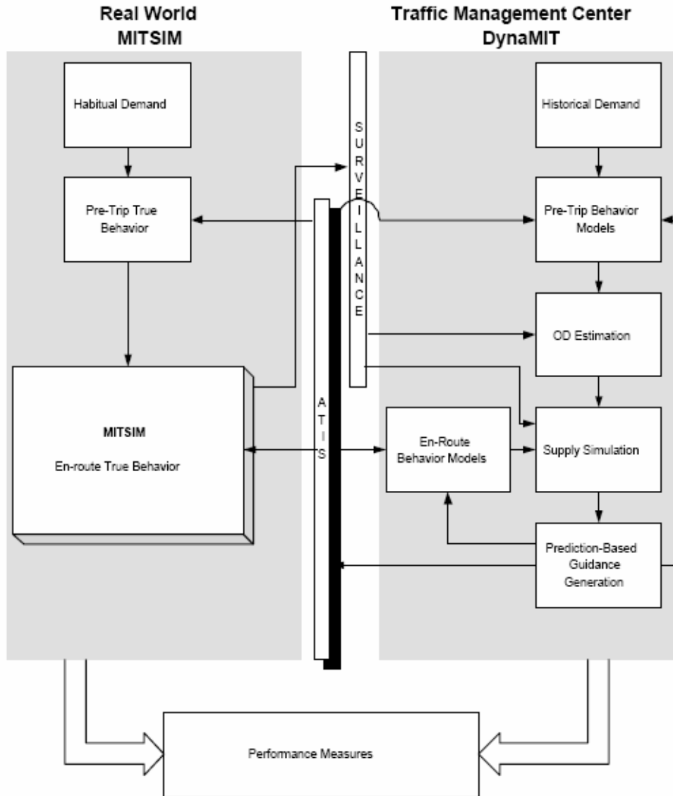
Figure 3-1 Dynamic Traffic Management Evaluation Framework using DynaMIT
