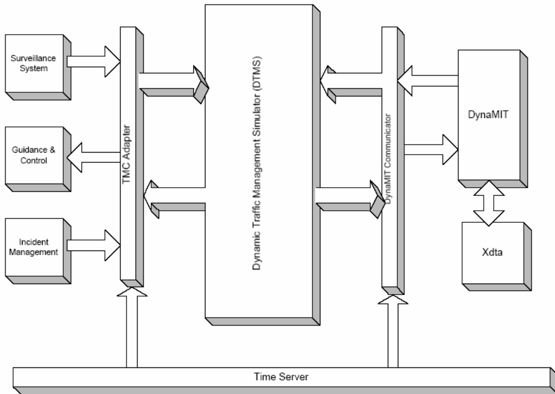
Figure 2-4 Modular Architecture for Dynamic Management Evaluation Framework
